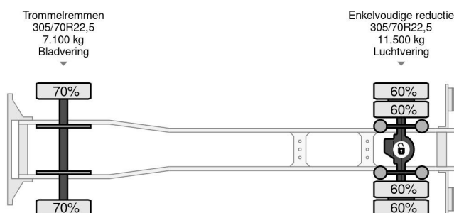
DAF 65 -180CF WITH HOOK-ARM CONTAINER SYST... 4x2
