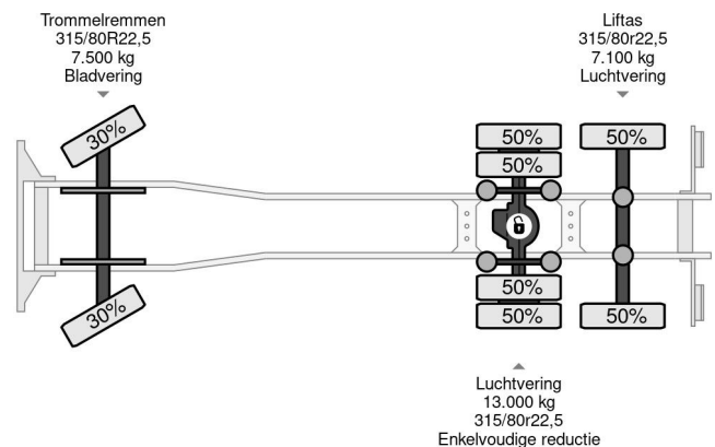
DAF 95.480 XF SPACECAB 6x2 WITH HOOK-ARM SYSTEM...
