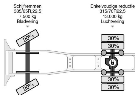
DAF XF 105.460 ATE SPACECAB AS-TRONIC (EURO ... 4x2
