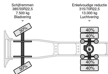
DAF XF 530 SUPERSPACECAB 4x2 TRACTOR UNIT (EURO...
