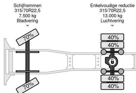
DAF XF 95.480 SPACECAB (EURO 4 / ZF16 MANUAL... 4x2 Referenznummer: SN 60134641 Z
