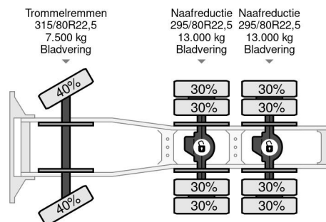
Renault R385 Major 6x4 SPRING SUSPENSION/LAMME (ZF... Referenznummer: SN 59970039 Z
