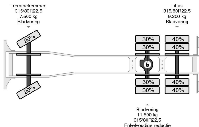
Scania R113-360 HL 6x2 FULL STEEL SUSPENSION BULK...
