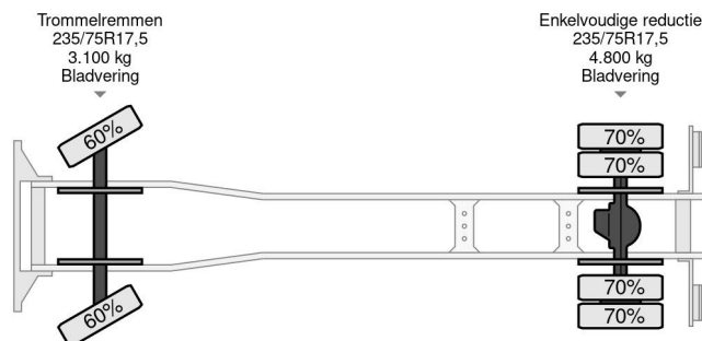
Mercedes-Benz LK 814 6-CILINDER FULL STEEL SUS... 4x2 Referentienummer: SN 57797229
