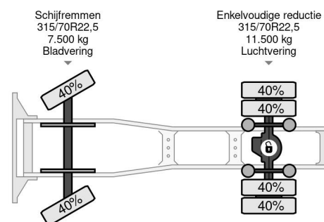
Renault T460 HIGH (EURO 6 / I-SHIFT / HYDRAULIC ... 4x2
