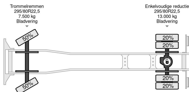
Scania R113-380 H 4X2 MEILLER KIPPER (FULL STEEL SU... Referentienummer: SN 55915961
