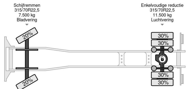
Mercedes-Benz Actros 1840 L (MP1) 4x2 STEEL-AIR SUSP...
