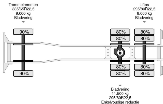
Scania P114-340 6x2 WITH MULTILIFT CONTAINERSYSTEM...
