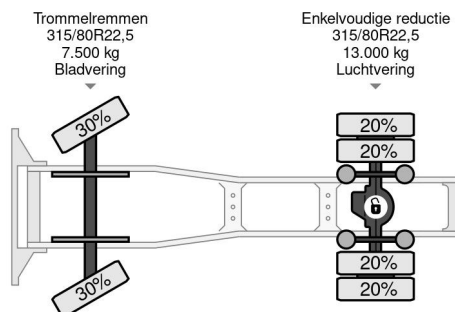
DAF 95.380 XF SPACECAB (EURO 2 (MECHANICAL ... 4x2 Referentienummer: SN 56068266 Z
