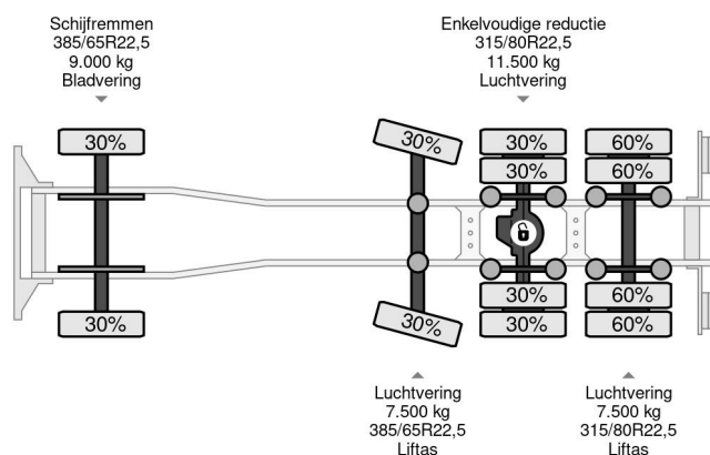
DAF XF 105.460 8x2 CHASSIS WITH MULTILIFT SYSTEM (... Referenznummer: SN 58952825
