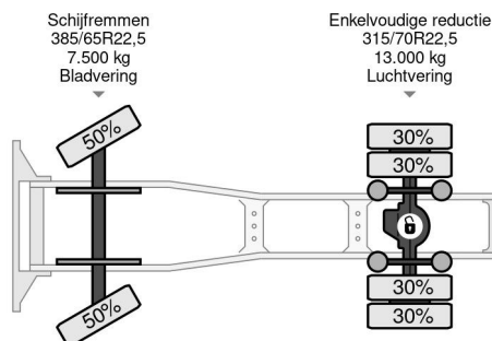
DAF XF 105.460 ATE SPACECAB (EURO 5 / AS-TRONIC GEARBOX / ZF-INTARDER / 870+430 LITER DIESEL TANK / AIRCONDITIONING) 4x2 Referentienummer: SN 60433089
